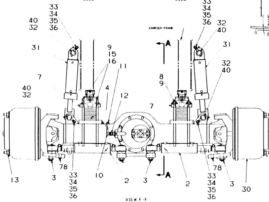
VIEW F-F ROTATED 90° CW
